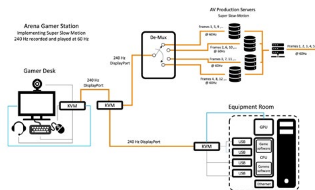
Figure 8: Signal-flow for super slow motion
