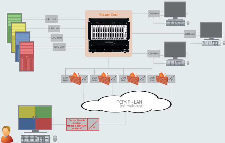
Operation with KVM matrix switch
